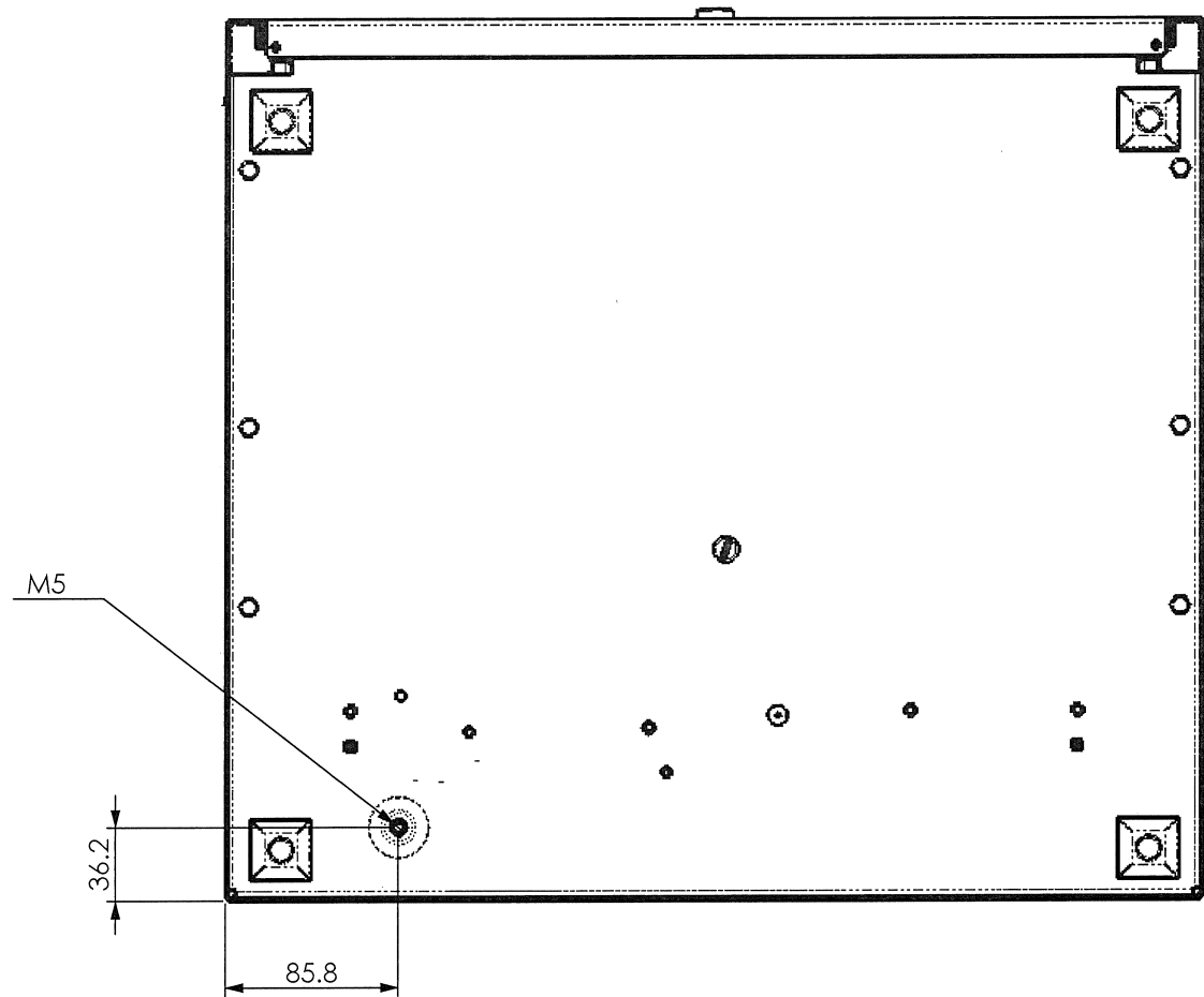
UNDERSIDE VIEW SHOWING FIXING DOWN HOLE POSITION
